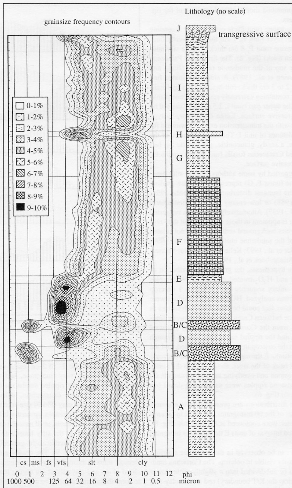
Figure 8. Contour plot of grain-size distribution in 60 samples across the K/T boundary in the Brazos 1 section. The samples are plotted in stratigraphic order but note that the true sample spacing is different. Therefore, the lithologic column represents lithologic expression of the samples in the correct stratigraphic order but has no vertical scale. The contours are at 1% spacing, and scores are computed for each 1/4 Phi class. A-J, lithologic units of Hansen et al. (1987). Abbreviations: cs = coarse sand, ms = medium sand, fs = fine sand, vfs = very fine sand, slt = silt, cly = clay.
